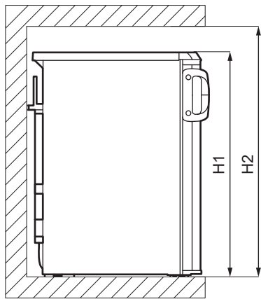
Overall dimensions 1
