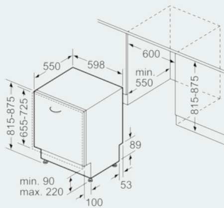
Dimensioned drawings
