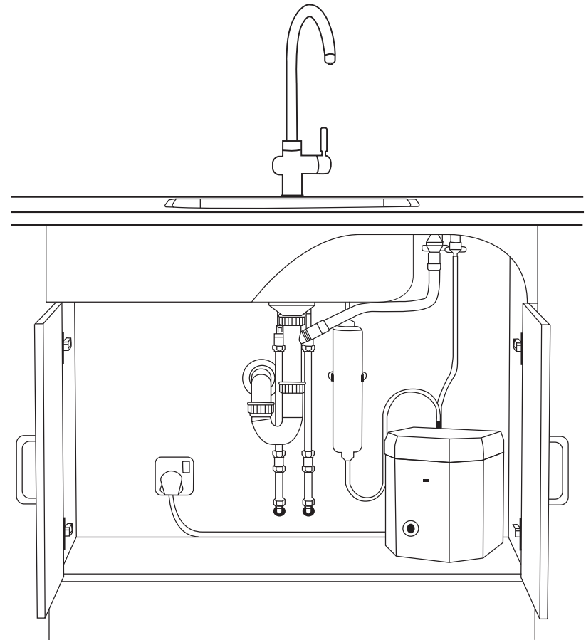
> Installation diagram for all One Stream Taps.
