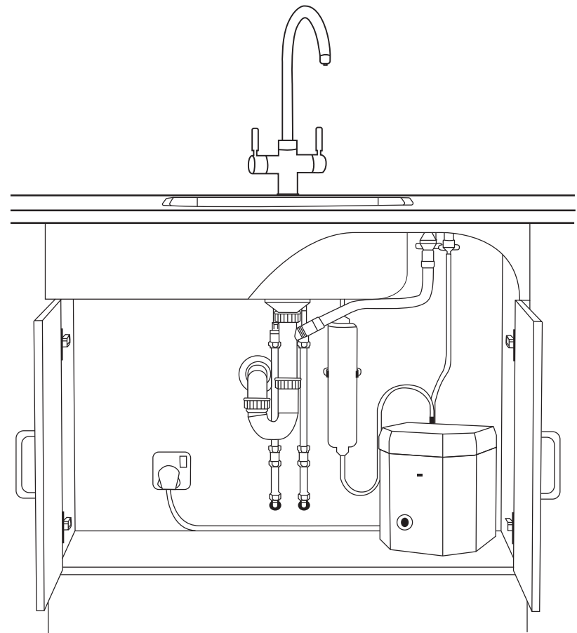
> Installation diagram for all Multiplex Taps.
